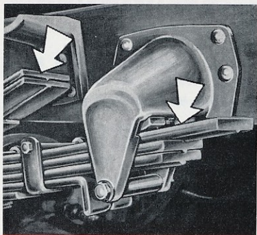
06-4 - Patins de ressort AR.
